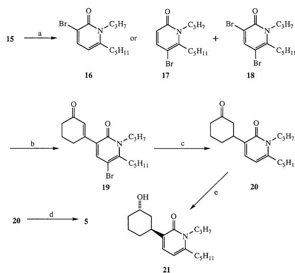
Scheme 3. (a) \text{Br}_2/\text{HOAc} , 25 °C; (b) n -BuLi/THF, -78^\circ\text{C} , then 3-ethoxycyclohex-2-en-1-one followed by \text{NH}_4\text{Cl} , or cyclohex-2-en-1-one, \text{Na}_2\text{CO}_3/\text{Pd}(\text{OAc})_2/\text{tri-}o\text{-tolylphosphine}/\text{DMF} ; (c) \text{H}_2(\text{g}) , 10% \text{Pd}(\text{C})/\text{EtOH}/40\text{psig} ; (d) \text{NaBH}_4/\text{EtOH} , 25 °C; (e) \text{K}(\text{sec-butyl})_3\text{BH}/\text{THF} , -78^\circ\text{C} to 25 °C, then \text{NaOH}/\text{H}_2\text{O}_2/\text{EtOH}/\text{H}_2\text{O} .
